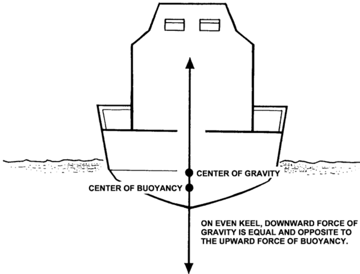
Figure 9-1 Stability in Equilibrium
