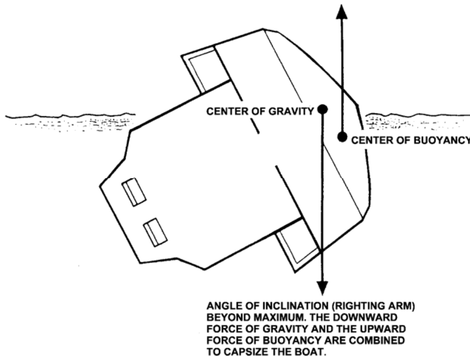
Figure 9-3 Righting Moment and Capsizing
