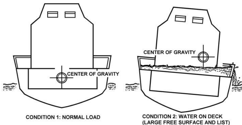
Figure 9-8 Effects of Water on Deck
