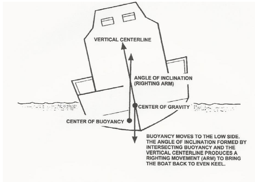
Figure 9-2 Heeling
