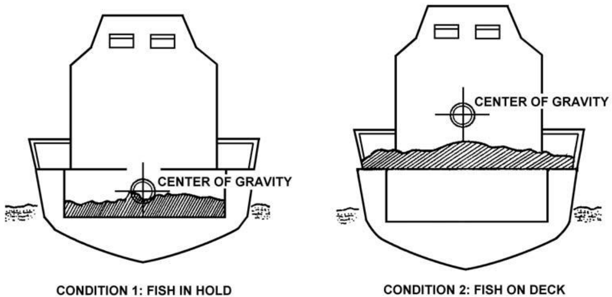
Figure 9-5 Effect of Load Weight
