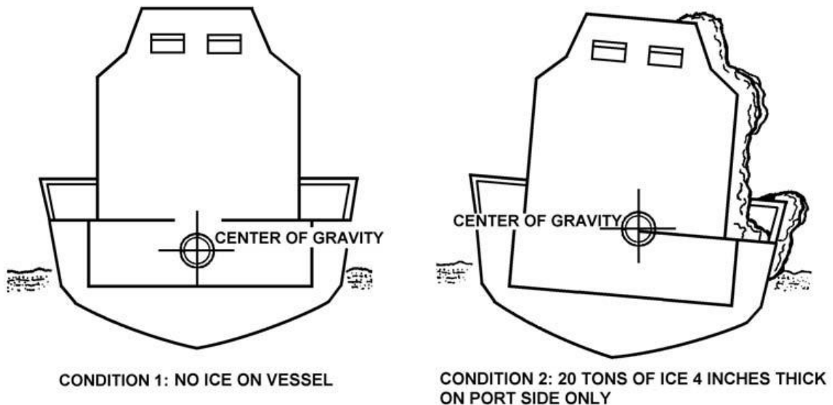
Figure 9-6 Effects of Icing
