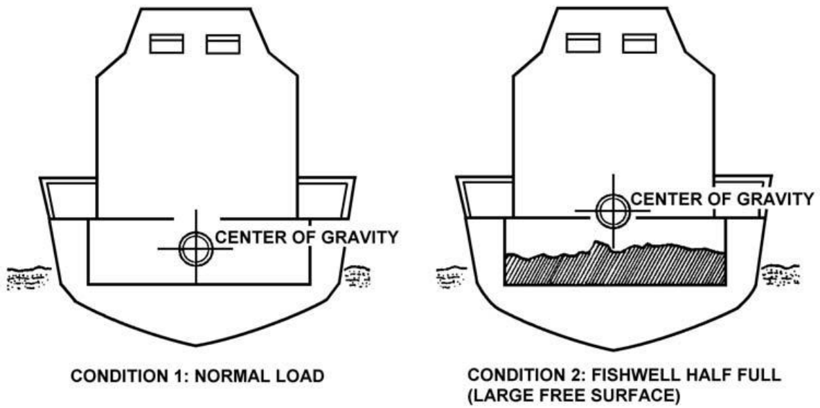
Figure 9-4 Effects of Free Surface
